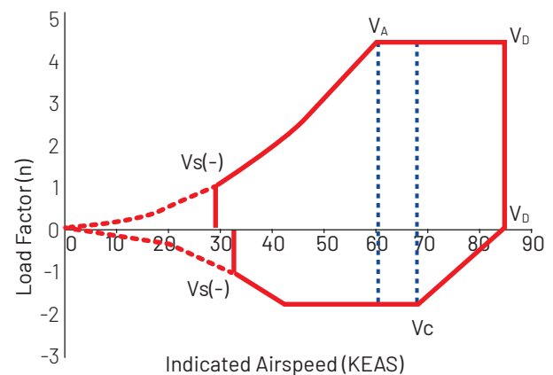
Figure 1. Schweizer SGU 2-22 Load factor
