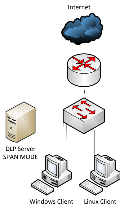
Figure 1. SPAN mode
