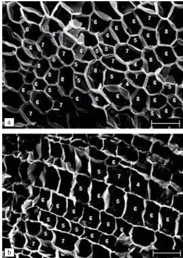
Figure 2 – Distribution of polygonal structure of Kielmeyera coriacea Mart. (“pau-santo”) cork. (a) Tangential section shows the number of vertices of each cell, and (b) non-tangential section of cork shows the number of sides (vertices) of each cell. Scales: (a) and (b) 100 µm.
