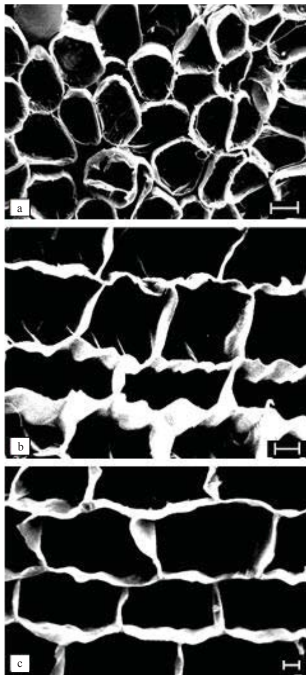
Figure 1 – General structure of Kielmeyera coriacea Mart. cork sections: (a) tangential section, (b) cross-section, (c) radial section. Scales: (a) 20µm, (b) 100 µm, (c) 20µm.
