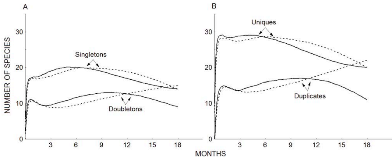
Figure 3. Numbers of bird species represented by one and two individuals (singletons and doubletons: A) and found in one and two samples (uniques and duplicates: B). Sampling was carried out using point counts in La Ventanilla-Tonameca lagoon, Oaxaca, continuous lines represent data from 20-minute counts and broken lines are from 10-minute counts.
