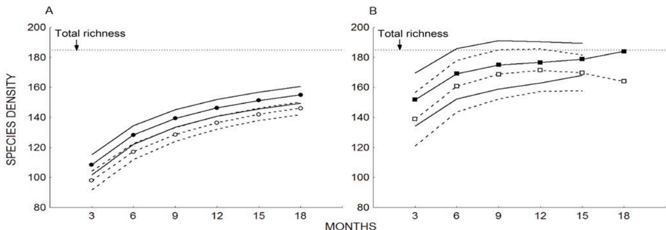
Figure 2. Sample-based rarefaction of bird data from La Ventanilla-Tonameca lagoon in Oaxaca. Species accumulation is a function of three-month intervals of sampling effort, with continuous and broken lines corresponding to 20 and 10-minute point counts, respectively. Circles (A) represent observed species density (SOBS) and squares (B) represent second order jackknife estimates (JK2). We generated the 84% CI analytically for SOBS (Mao Tau) and with 1,000 randomizations for JK2.
