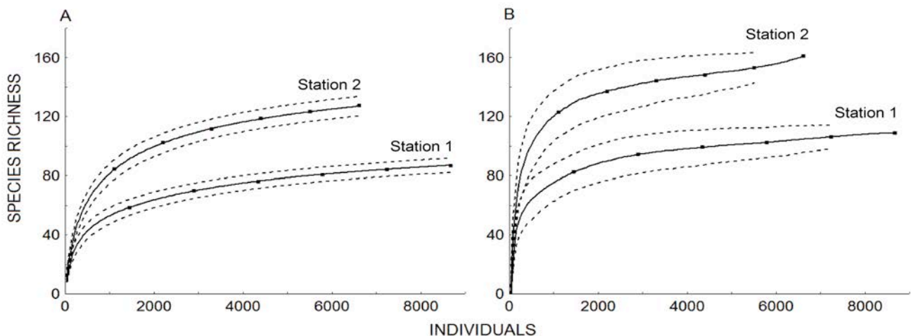
Figure 4. Comparison of species richness in contrasting habitat types in the La Ventanilla-Tonameca coastal lagoon, Oaxaca. Station 1 corresponds to a mangrove forest and station 2 to a seasonally tidal estuary without mangrove trees. Data was collected using 20-minute point counts, the abscissa is re-scaled to individuals, and three-month sampling intervals are indicated on each plot. Broken lines represent 84% CI , generated analytically for observed species richness (SOBS: A) and with 1,000 randomizations for second order jackknife estimates (JK2: B).
