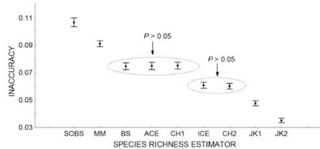
Figure 1. Relative inaccuracy of nine estimates of bird richness in the coastal lagoon La Ventanilla-Tonameca, Oaxaca. We obtained the nine estimates using standardized sampling (SOBS) and eight richness estimators: Incidence-based Coverage Estimator (ICE), Abundance-Based Coverage Estimator (ACE), Chao 1 (CH1), Chao 2 (CH2), first order jackknife (JK1), second order jackknife (JK2), Bootstrap (BS) and Michaelis-Menten (MM). We calculated the estimate inaccuracies using an empirical estimate of total species richness: (\text{estimate} - \text{total})/\text{total} . Statistical intervals were calculated with the standard error and P values refer to comparisons between estimates using Mann-Whitney U tests. We found statistical difference at a 0.05 significance level between all estimators except those circled.
