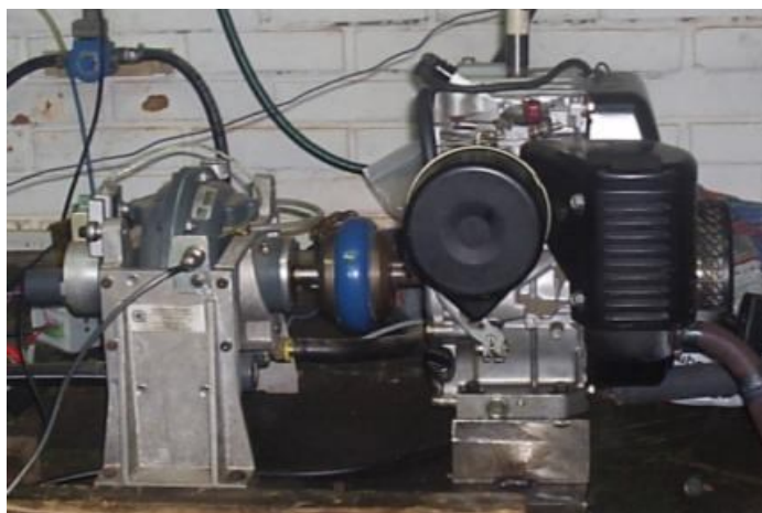
Figure 3. Experimental setup
