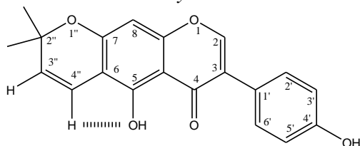
Figure 1: Compound 1
