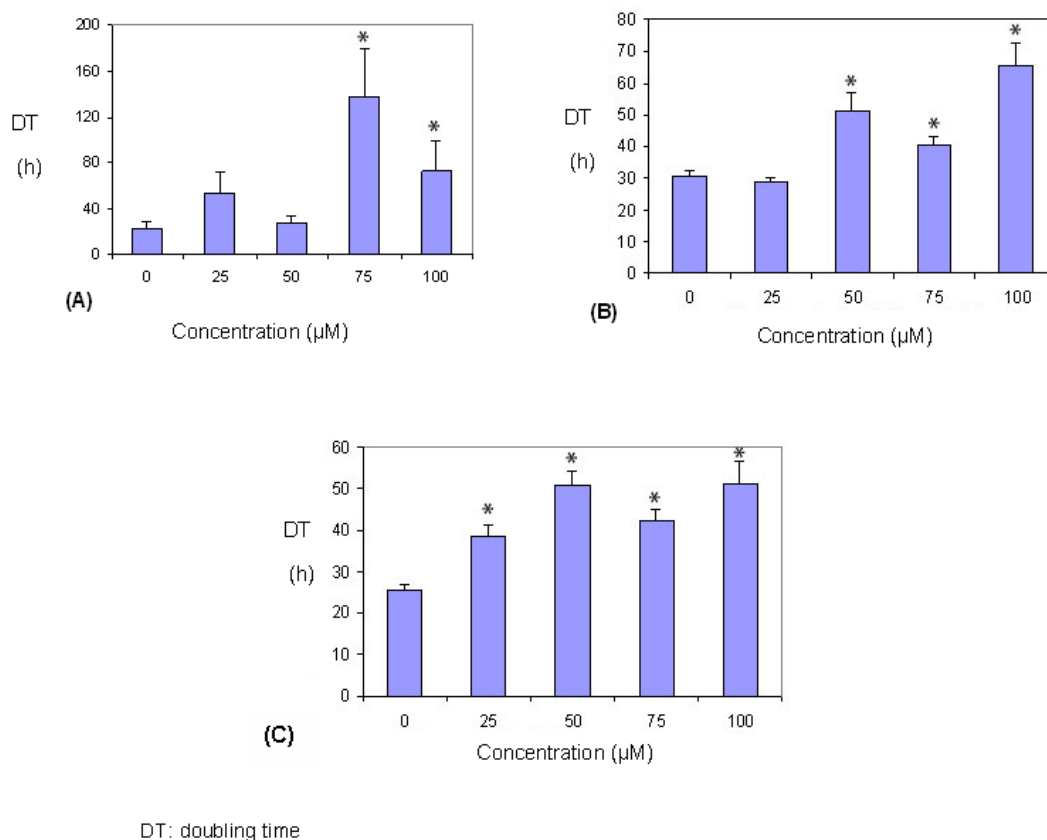
Figure 2: Effect in the time of doubling on UCHT1 cells treated with compounds obtained from resin of Heliotropium filifolium and derivatives semi-synthetic. The concentrations of the compounds are expressed in \mu M. The results correspond to the mean \pm EE of the values of three independent experiments in triplicate. (A) Cells treated with different concentrations of filifolinol * p < 0.05 respect to control. (B) Cells treated with different concentrations of filifolinone * p < 0.01 respect to control. (C) Cells treated with different concentrations of filifolinoic acid * p < 0.01 respect to control.
