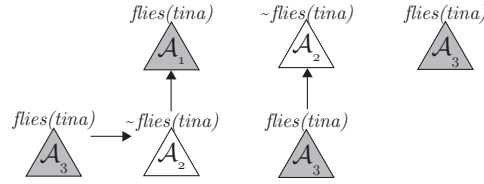
Figure 1. D-trees for flies(tina)
