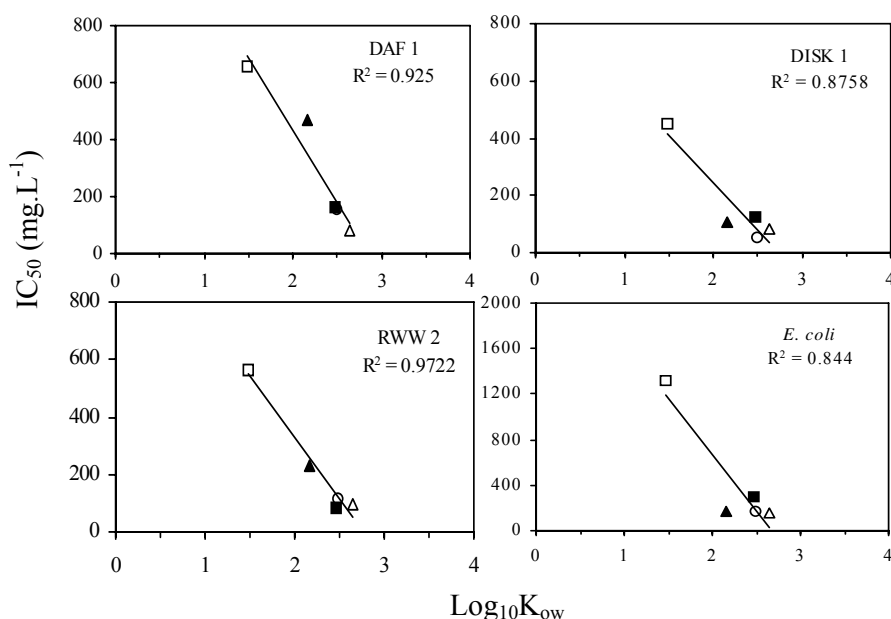
Figure 5. Acute toxicity of five phenols against Log 10 K ow for \beta -galactosidase activity of Pseudomonas sp. DAF1, Pseudomonas sp. RWW2, Bacillus sp. DISK1 and Escherichia coli . The linear regression relationships are based on: phenol □; 2-chlorophenol ▲; 3,5-dimethylphenol ■; 4-bromophenol Δ and 4-chlorophenol ○.
