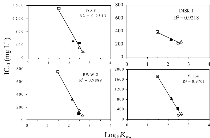
Figure 4. Acute toxicity of five phenols against Log K ow for \alpha -glucosidase activity of Pseudomonas sp. DAF1, Pseudomonas sp. RWW2, Bacillus sp. DISK1 and Escherichia coli . The linear regression relationships are based on: phenol □; 2-chlorophenol ▲; 3,5-dimethylphenol ■; 4-bromophenol Δ and 4-chlorophenol ○.
