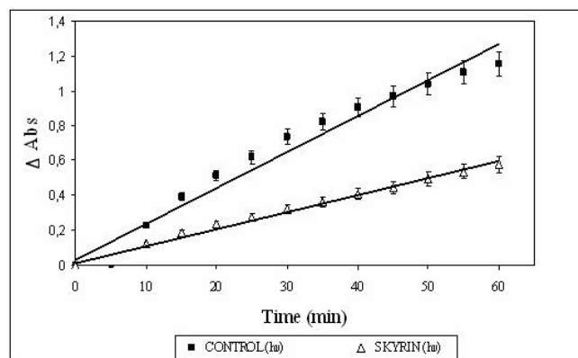
Figure 7. UV monitoring at 440 nm of the singlet oxygen quenching by addition of skyrin (control without skyrin) during the irradiation of rose bengal in the presence of histidine and p-nitrosoaniline. Data in the inset are shown as mean \pm SD ( n = 3 ).
