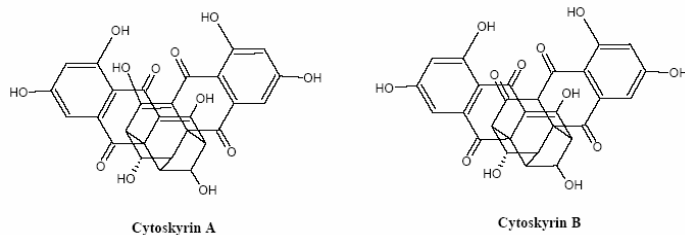
Figure 1. Structures of the cytoskyrin A and B.
