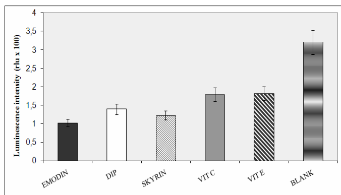
Figure 5. Quenching effect of the luminol chemiluminescence ( \text{H}_2\text{O}_2 = blank) observed for emodin, dipyrindamole (DIP), skyrin, vitamin C and E. Data in the inset are shown as mean \pm SD ( n = 3 ).
