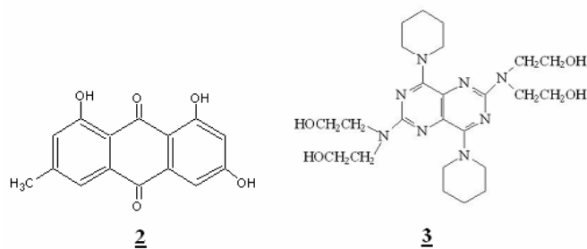
Figure 3. Structures of the antioxidants emodin (2) and dipyrindamole (3).
