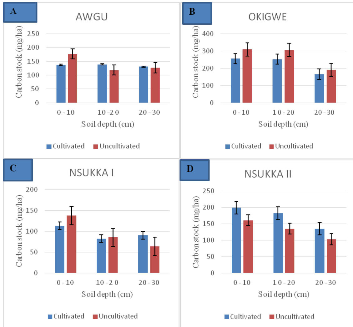
Figure 1. Distribution of soil carbon stock across varying top soil depths of the study locations in Southeastern Nigeria: Awgu (A), Okigwe (B), Nsukka I (C), and Nsukka II (D).
