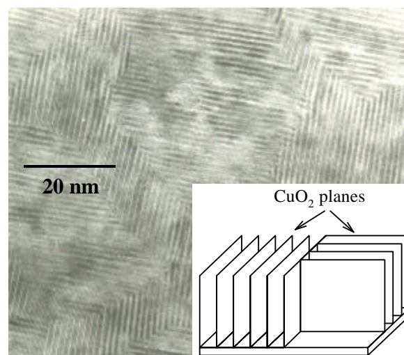
Fig 2: Plan view HRTEM image of an a-axis EBCO film. Inset shows a sketch of the \text{CuO}_2 planes indicating the domain microstructure
