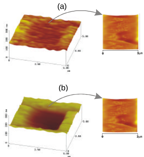
Fig. 7. AFM images of the wear mark produced (a) by one wear cycle and (b) after 15 wear cycles.
