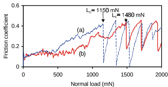
Fig. 5. Friction coefficient vs normal load data obtained from the microscratch measurements on the coatings: (a) 24% CH 4 WC on steel, (b) 24% CH 4 WC/W on steel. The arrows indicate the adhesive failure of the coatings at the critical load values ( L_c ).
